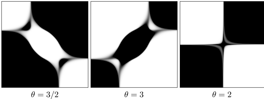
Fig. 5.2: Comparison of optimal coupling \gamma^* for different values of \theta .
