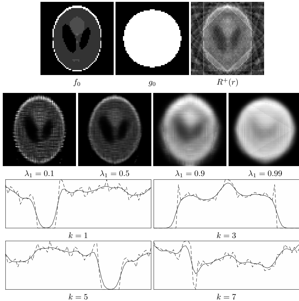
Fig. 3.3: Example of reconstructions from partial Radon measurements. The two bottom rows show the input transforms r_k = R_{\theta_k}(f_0) (dashed curves) and the recovered Radon transforms R_{\theta_k}(f) where f solved 3.9 (plain curves), for a few values of k .
