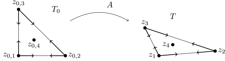
Fig. 4: The Hermite \mathcal{P}_3 interpolation is determined by 4 control nodes which impose the values of the polynomial at z_1, \dots, z_4 and the gradient at z_1, z_2, z_3 . Those nodes are the three vertices and the barycenter. Each element T is the image of the reference element T_0 through some affine map A .
