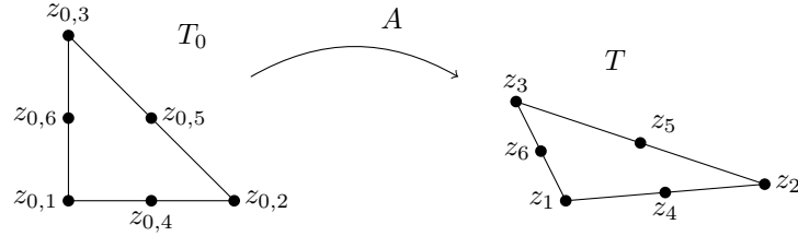
Fig. 3: The Lagrange \mathcal{P}_2 interpolation is determined by 6 control nodes which impose the values of the polynomial at z_1, \dots, z_6 . Those nodes are the three vertices and the middle of each edge. Each element T is the image of the reference element T_0 through some affine map A .
