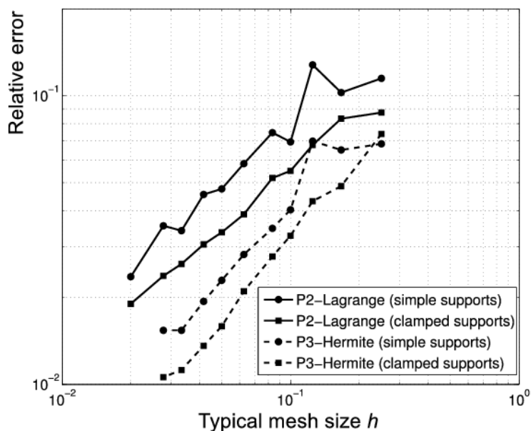
Fig. 5: Relative error versus mesh size for the square plate problem for the \mathcal{P}_2 Lagrange and \mathcal{P}_3 Hermite element for different boundary conditions
