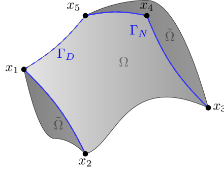
Fig. 1: The domain \Omega is piecewise C^3 regular, i.e. C^3 except at a finite number of points \{x_1, \dots, x_J\} . The (relaxed) Neumann boundary condition is imposed on \Gamma_N = (\partial\Omega) \cap \tilde{\Omega} where \tilde{\Omega} \supset \Omega is a piecewise C^3 domain.
