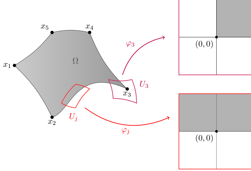
Fig. 2: The local charts used to smooth the function u in Proposition 6.
