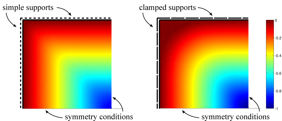
Fig. 6: Representation of the obtained failure mechanism u for the square plate problem with simple supports (left) and clamped supports (right) using the \mathcal{P}_2 Lagrange element
