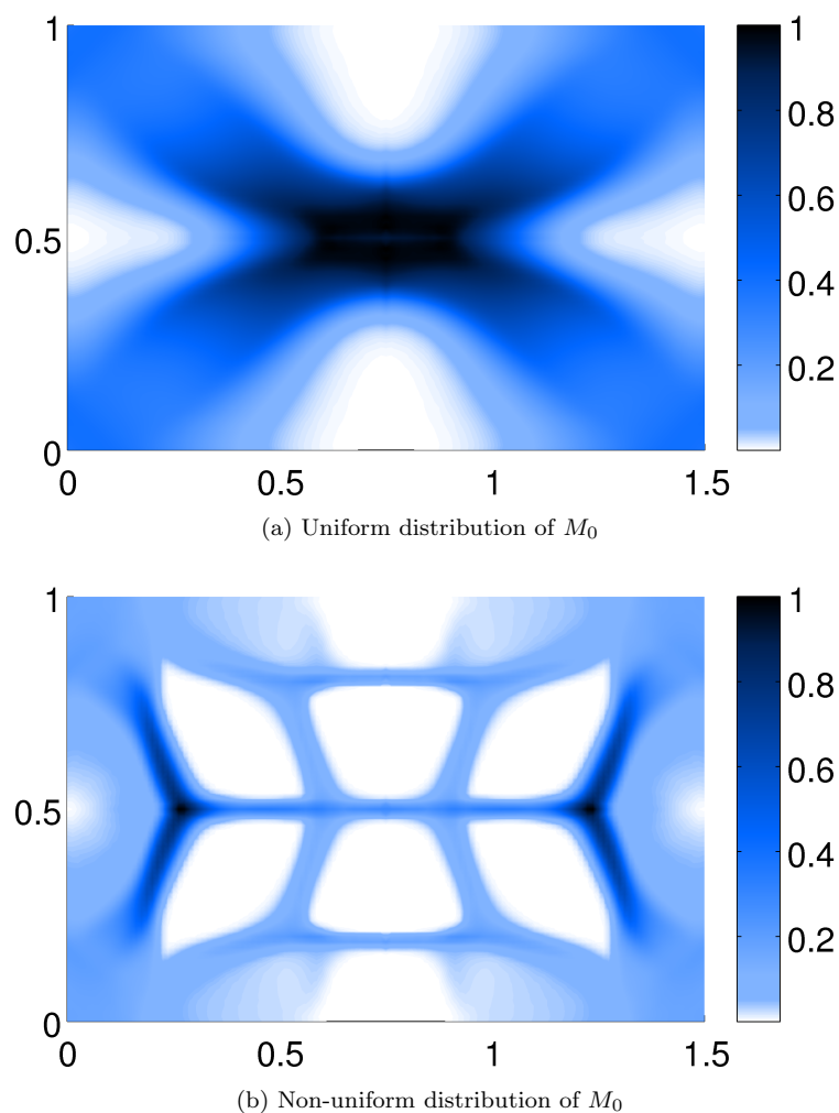
Fig. 9: Comparison of the relative distribution of \Pi(D^2u(x)) obtained for a non-uniform and a uniform distribution of the strength parameter
