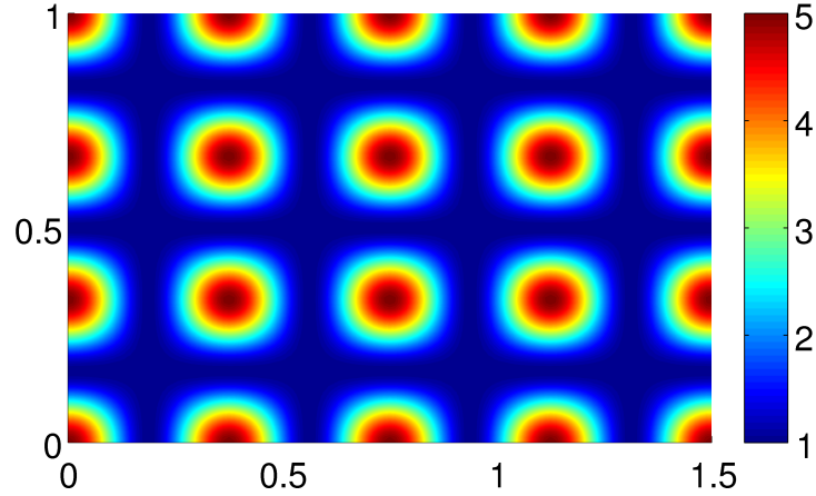
Fig. 7: Representation of the variation of the uniaxial strength in bending M_0(x_1, x_2) for the non-uniform example
