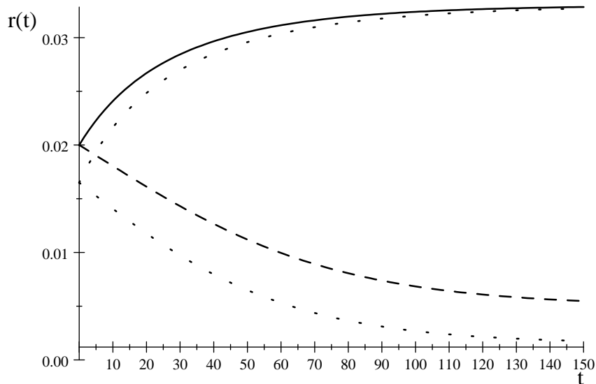
Figure 1: \delta = 0.02 , n = 0.013 . Solid curve shows r(t) for \sigma = 0.06 and g = 0 . Dashed curve shows r(t) for \sigma = 0.005 and g = 0 . The two dotted curves increase g to 0.0035
