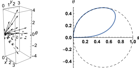
Figure 2. Left: Finite difference stencil of (10) and (17) with dashed arrows when \langle \dot{\mathbf{e}}_i^\theta, (0, 0, 1)^T \rangle < 0 . Right: Unit vectors in tangent space for EM elastica model, and the variant with convexity prior. Set of all (\dot{s}, \dot{\theta}) such that \mathcal{F}^C(\mathbf{x}, (\dot{s}\vartheta_\theta, \dot{\theta})) = 1 (solid line), and likewise for \mathcal{F}^{\text{EM}} (dashed line)
