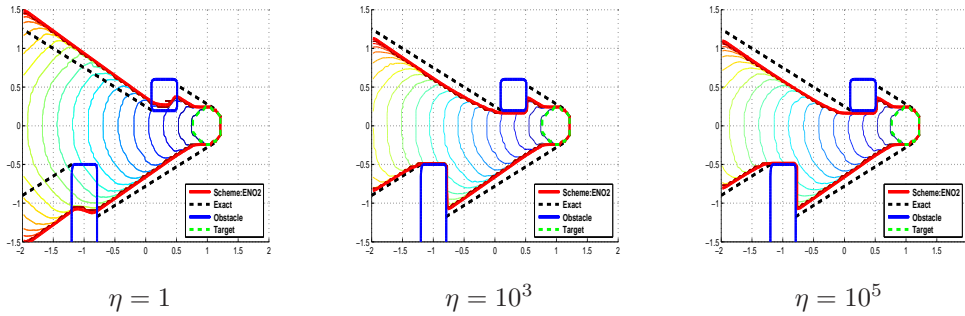
FIG. 6.5. (Example 2) Approach (2.9) with various \eta parameters, and M_{x_1} = M_{x_2} = 100 .
