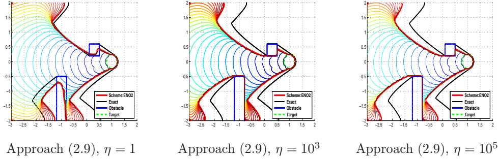
FIG. 6.8. (Example 3) Approach (2.9) with various \eta parameters, M_{x_1} = M_{x_2} = 100 .
