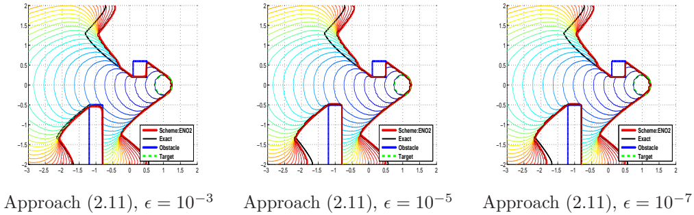
FIG. 6.9. (Example 3) Penalisation approach (2.11) with various \epsilon parameters, M_{x_1} = M_{x_2} = 100 .
