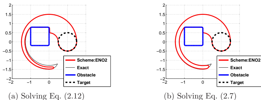
FIG. 6.3. (Example 1) Backward reachable set, t = 0.75 , with second order ENO2 scheme, (a) solving Eq. (2.12) and (b) solving Eq. (2.7), M_{x_1} = M_{x_2} = 100 .
