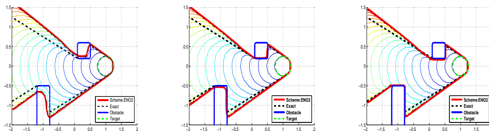
Approach (2.11), \epsilon = 10^{-2} Approach (2.11), \epsilon = 10^{-3} Approach (2.11), \epsilon = 10^{-5}
