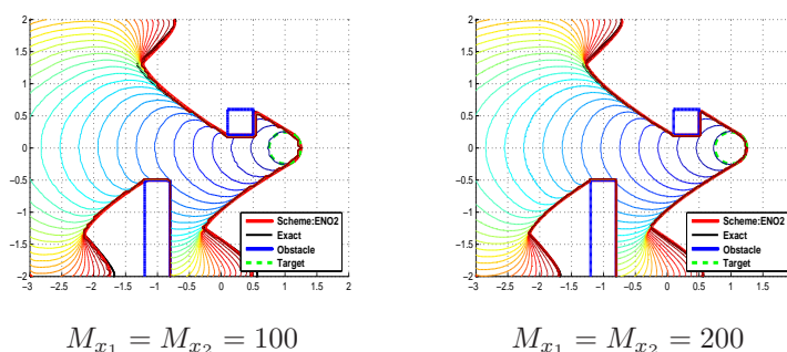
FIG. 6.7. (Example 3), obstacle approach (2.7).
