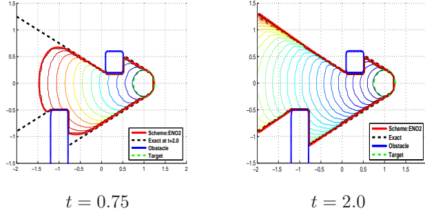
FIG. 6.4. (Example 2) Backward reachable set for the Zermelo problem with obstacle, at t = 0.75 (left) and at t = 2.0 (right). The computational domain is [-2, 2]^2 , and M_{x_1} = M_{x_2} = 100 .
