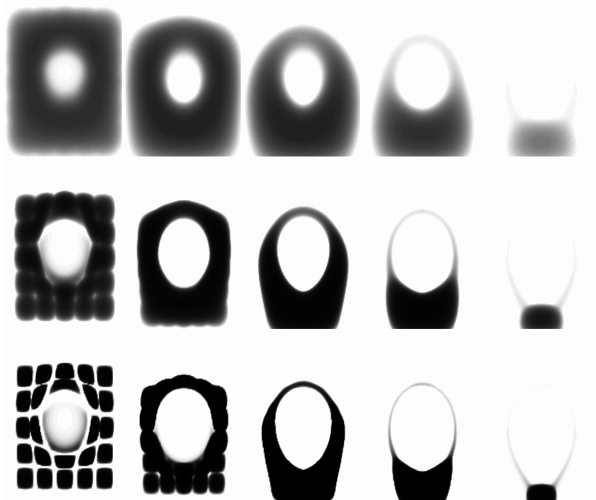
Fig. 4 Simulation of crowd motion under congestion using the gradient flow formulation. The congestion term is given by \beta\mathcal{U}_1 (see Equation (5.65)), for various values of \beta . From top to bottom, \beta is set to 10^{-k} for 0 \leq k \leq 2 .
