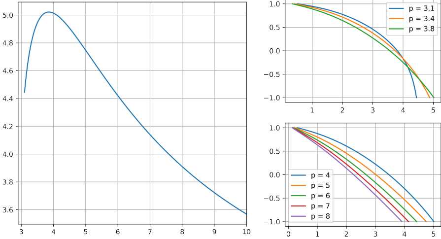
Figure 4. Radial case with d = 3 and m = 1 . (Left) The function p \mapsto \alpha_{\star}^{\text{rad}, (\kappa=1)}(p) reaches its maximum at p \approx 3.86 . (Right) The maps \alpha \mapsto \Lambda_D^{\text{rad}, (\kappa=1)}(\alpha, p) for values of p corresponding either to p < 3.86 (top) or p > 3.86 (bottom).
