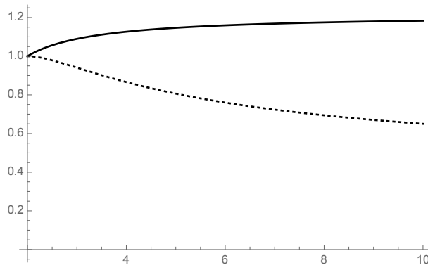
FIGURE 4. The curves p \mapsto \lambda_1 (dotted) and p \mapsto \lambda_1^* (plain) differ [Erratum: this figure differs from the published version as there was an incorrect term in the original numerical code].
