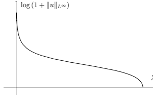
FIGURE 1. \varepsilon = 0 , the bifurcation diagram in the critical case.
