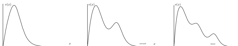
FIGURE 6. Functions corresponding to the first three turning points to the right in the previous bifurcation diagram, with \varepsilon = 0.2 , after the transformation:
