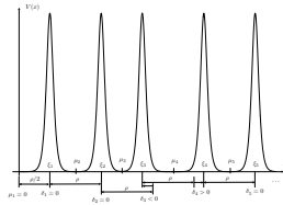
FIGURE 4. The function V is defined by V = \sum_{i=1}^k V_i where V_i = U_i + \pi_i , U_i(x) = U(x - \xi_i) and \pi_i(x) = -U(\xi_i)e^{-x} . The function U is the unique solution of (2.5). The intervals are defined by \xi_1 = \frac{\rho}{2} + \delta_1 and \xi_i = \xi_{i-1} + \rho + \delta_i for i = 2, \dots, k , where \rho = -\log \varepsilon tends to +\infty and |\delta_i| \leq K for some fixed constant K .
