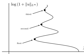
FIGURE 5. The bifurcation diagram corresponding to N = 5 , p = 7/3 and \varepsilon = 0.2 , with the first three turning points to the right of the bifurcation diagram.
