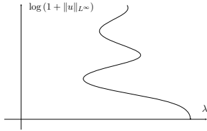
FIGURE 2. \varepsilon > 0 , the bifurcation diagram in the supercritical case (here \varepsilon = \varepsilon_0 = 0.2 ).
