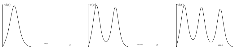
FIGURE 7. Functions corresponding to the first three turning points to the right in the bifurcation diagram, corresponding now to \varepsilon = 0.01 .
