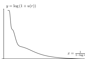
FIGURE 8. A 3-bubble solution u of (1.1) corresponding to the three bumps solution v of Figure 7, with \varepsilon = 0.01 . Appropriate scales have been chosen.
