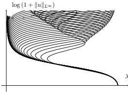
FIGURE 3. Approximating the critical case: \varepsilon = 2^{-q}\varepsilon_0 , N \ni q \rightarrow \infty , \varepsilon_0 = 0.2 .
