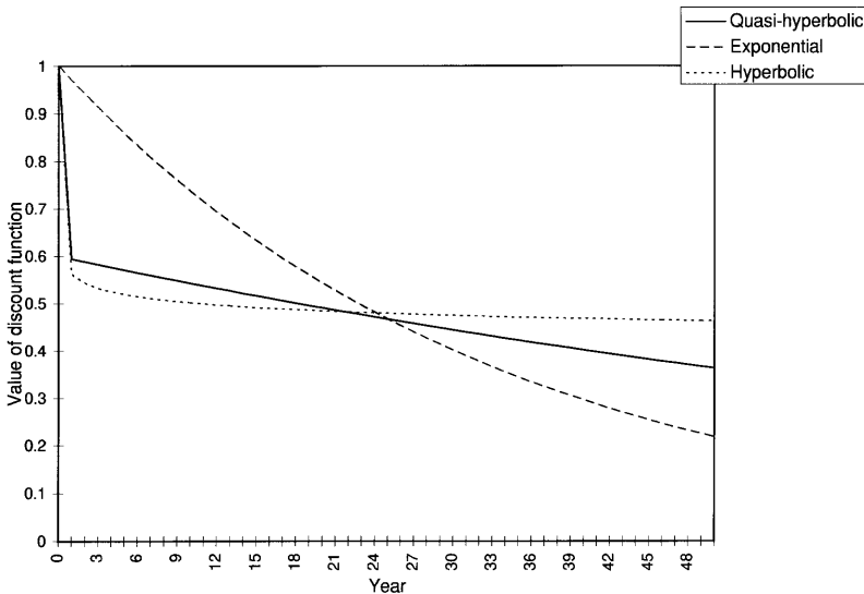
FIGURE I Discount Functions
