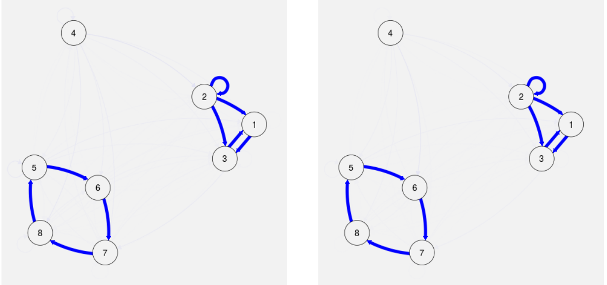
(b) Results for scenario 2 over the 25 simulated datasets. Posterior estimation of the interaction graph for T = 10 on the left and T = 20 on the right. Level of grey and width of the edges are proportional to the posterior estimated probability of \frac{1}{25} \sum_{sim=1}^{25} \mathbb{P}(\delta^{(k,\ell)} = 1 | (N_t^{sim})_{t \in [0,T]}) .
