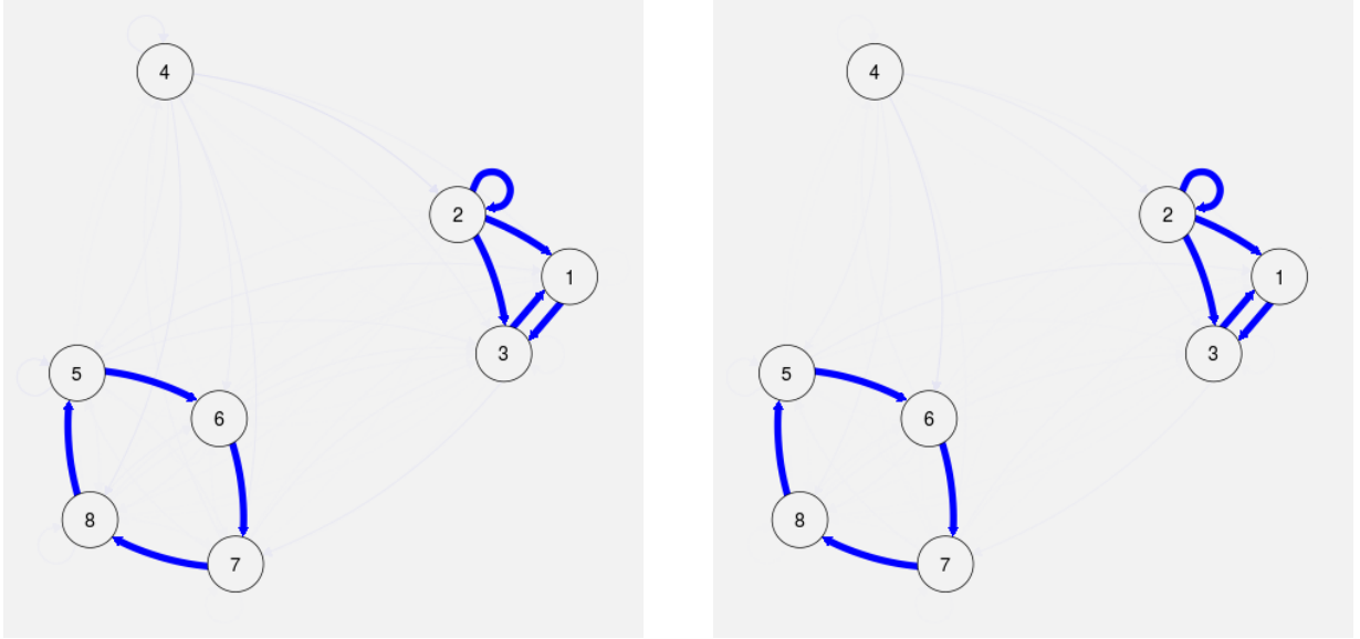
(a) Results for scenario 2 for one given dataset. Posterior estimation of the interaction graph for T = 10 on the left and T = 20 on the right, for one randomly chosen dataset. Level of grey and width of the edges proportional to the posterior estimated probability of \mathbb{P}(\delta^{(k,\ell)} = 1 | (N_t^{sim})_{t \in [0,T]}) .
