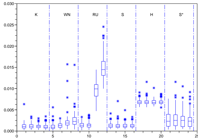
Figure 4: Boxplots of the ISE for g_d over 100 simulations for the 6 methods and the 4 different values of d . A column, delimited by dashed lines, corresponds to one method (respectively K , WN , RU , S , H , S* ). Inside this column, from left to right, one can find for the same method the boxplots of the ISE for respectively d = 10, 30, 50 and 70 .
