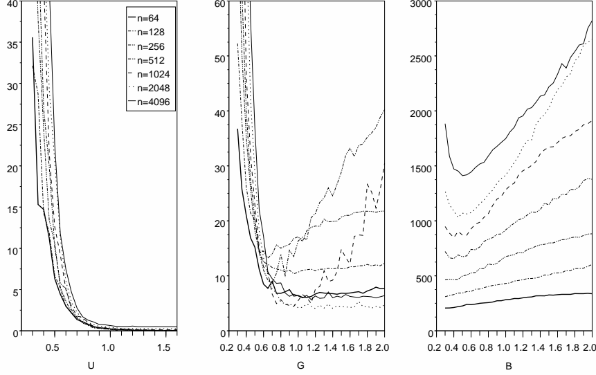
Figure 1: n \times MIS E_n(\gamma) for (U) f = \mathbb{1}_{[0,1]} (the Haar basis is used) ; (G) f is the Gaussian density with mean 0.5 and standard deviation 0.25 (the Spline basis is used) ; (B) f is the renormalized Bumps signal (the Spline basis is used)
